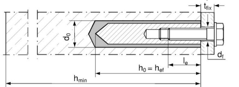
fischer internal threaded anchor RG MI Pre-positioned anchor only
