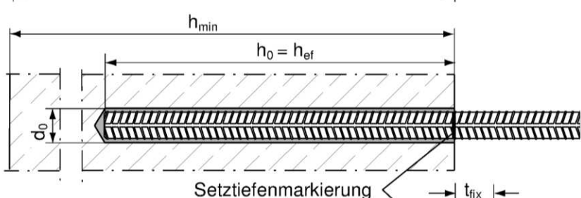
Reinforcing bar
